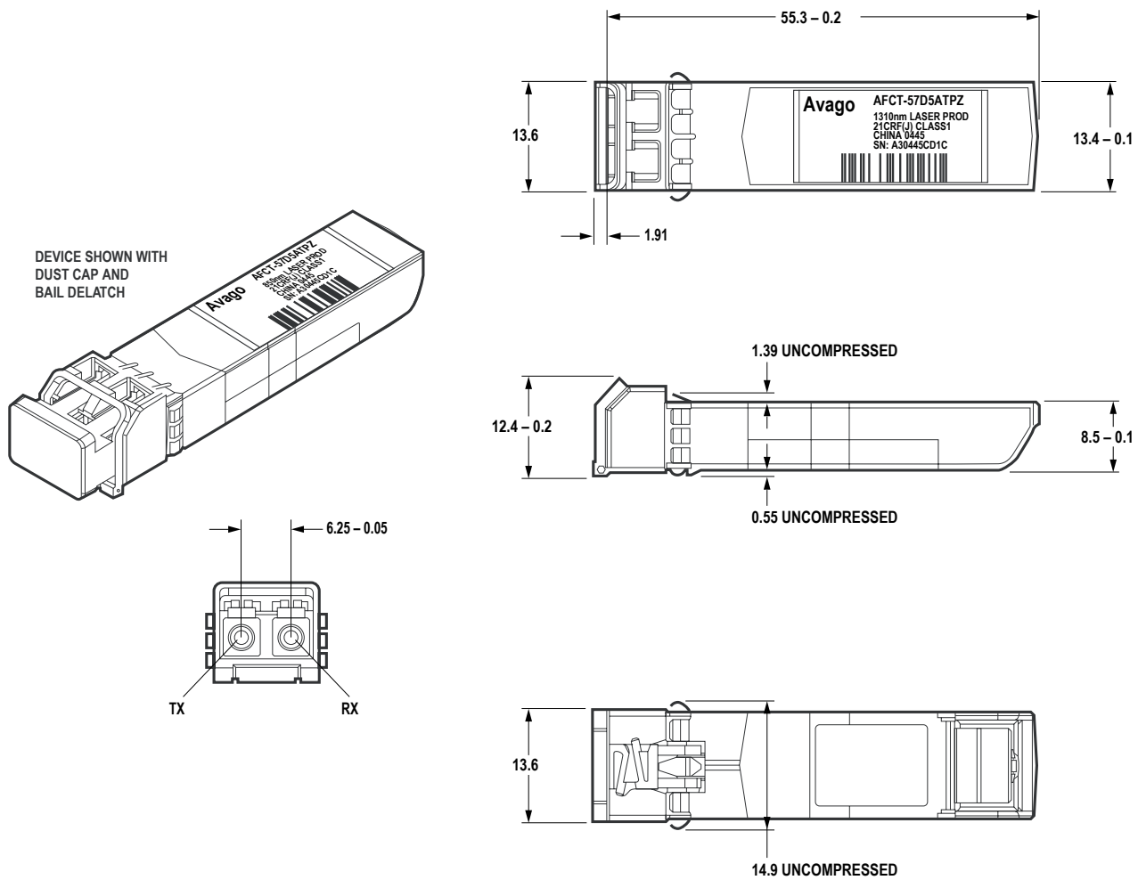
Figure 5. Module drawing.
